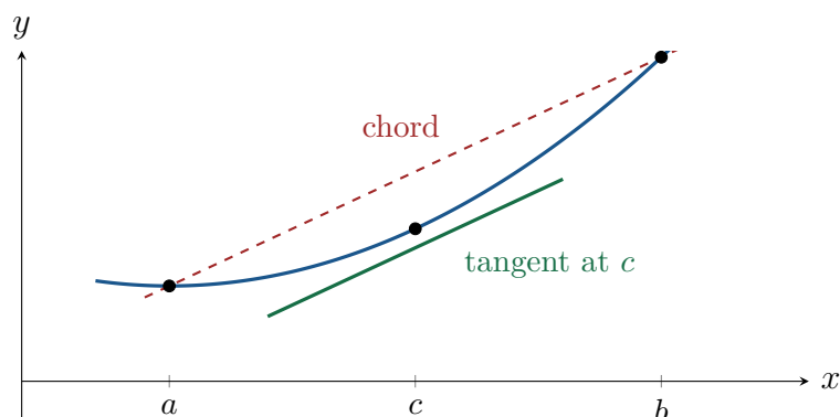
Figure 2: Lagrange's Mean Value Theorem. Somewhere inside, the tangent is parallel to the chord.
