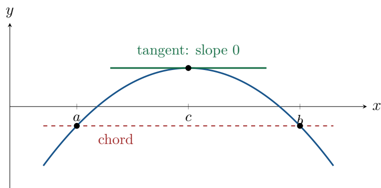
Figure 1: Rolle’s Theorem. The chord is horizontal because f(a) = f(b) , and somewhere inside the tangent is horizontal too.
